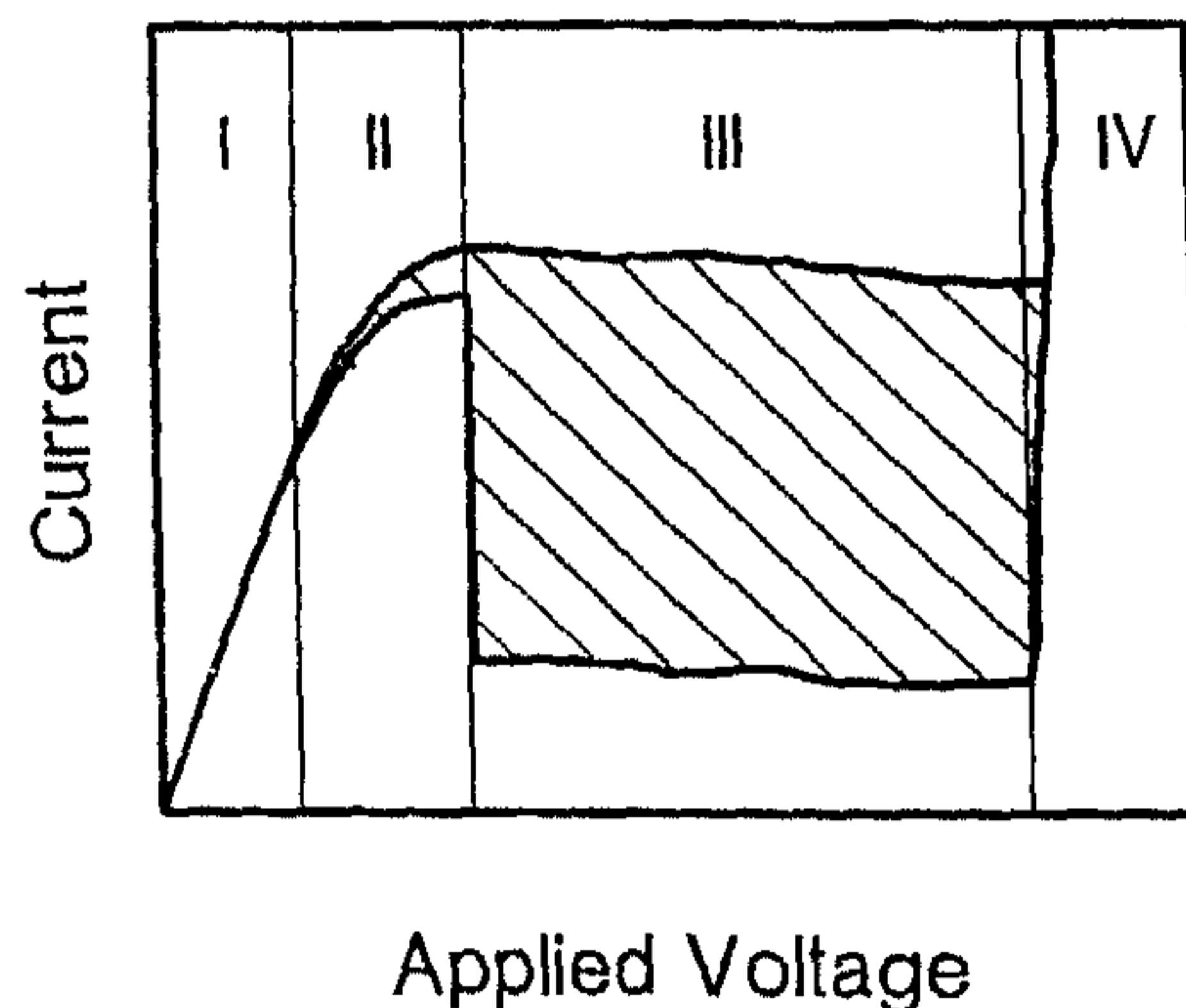
Figure 2. A typical I(V_{appl}) -characteristic of a sample, showing four different regimes: i, ohmic; ii, small sinusoidal oscillations; iii, large pulse-like oscillations; iv, electrical breakdown. The upper and lower curves represent the maximum and minimum current between which the system oscillates (hatched area).
