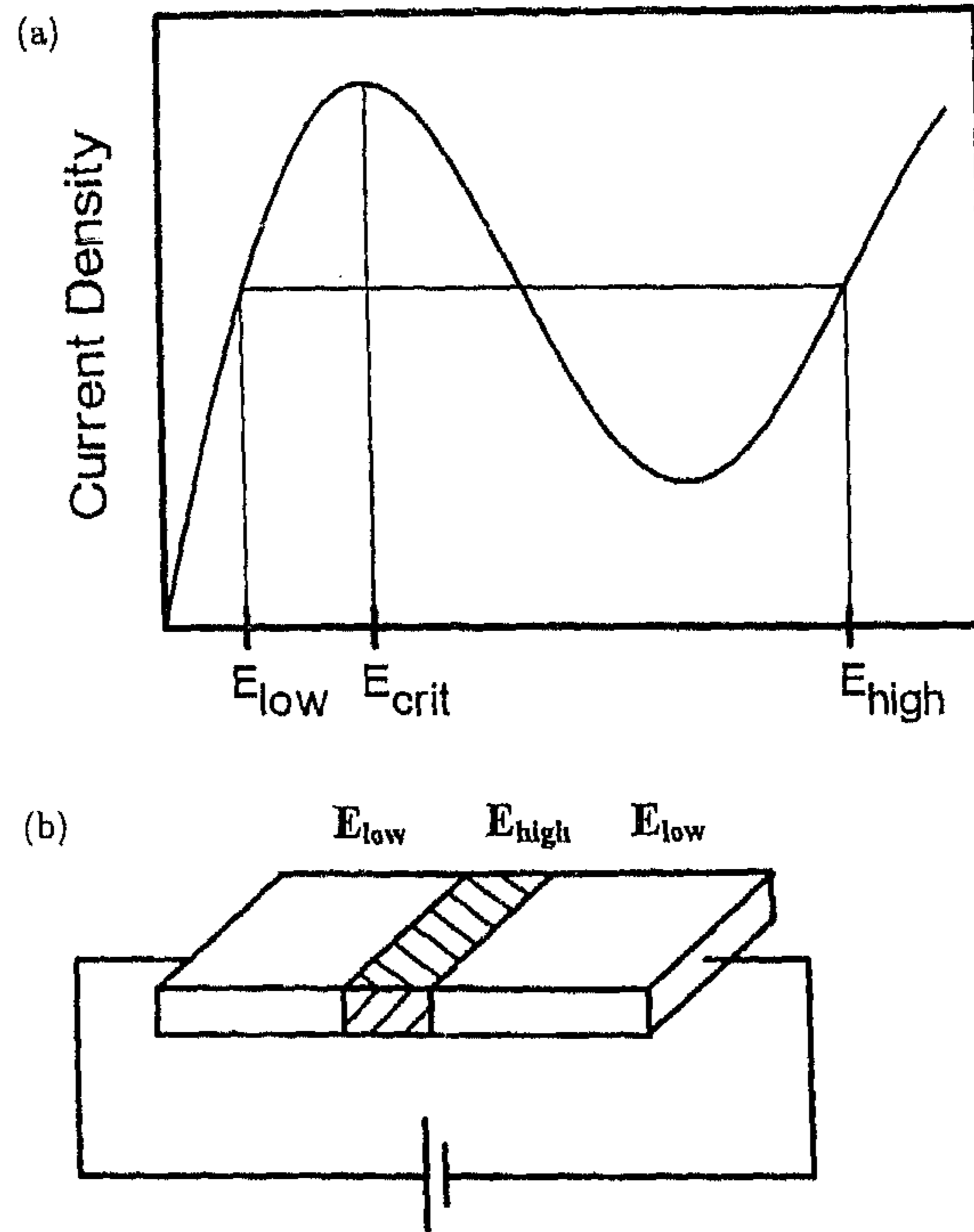
Figure 1. A schematic non-linear j(E) -characteristic with an N-shaped negative differential conductivity (a) which leads to the topological partition of a sample into domains (b).
