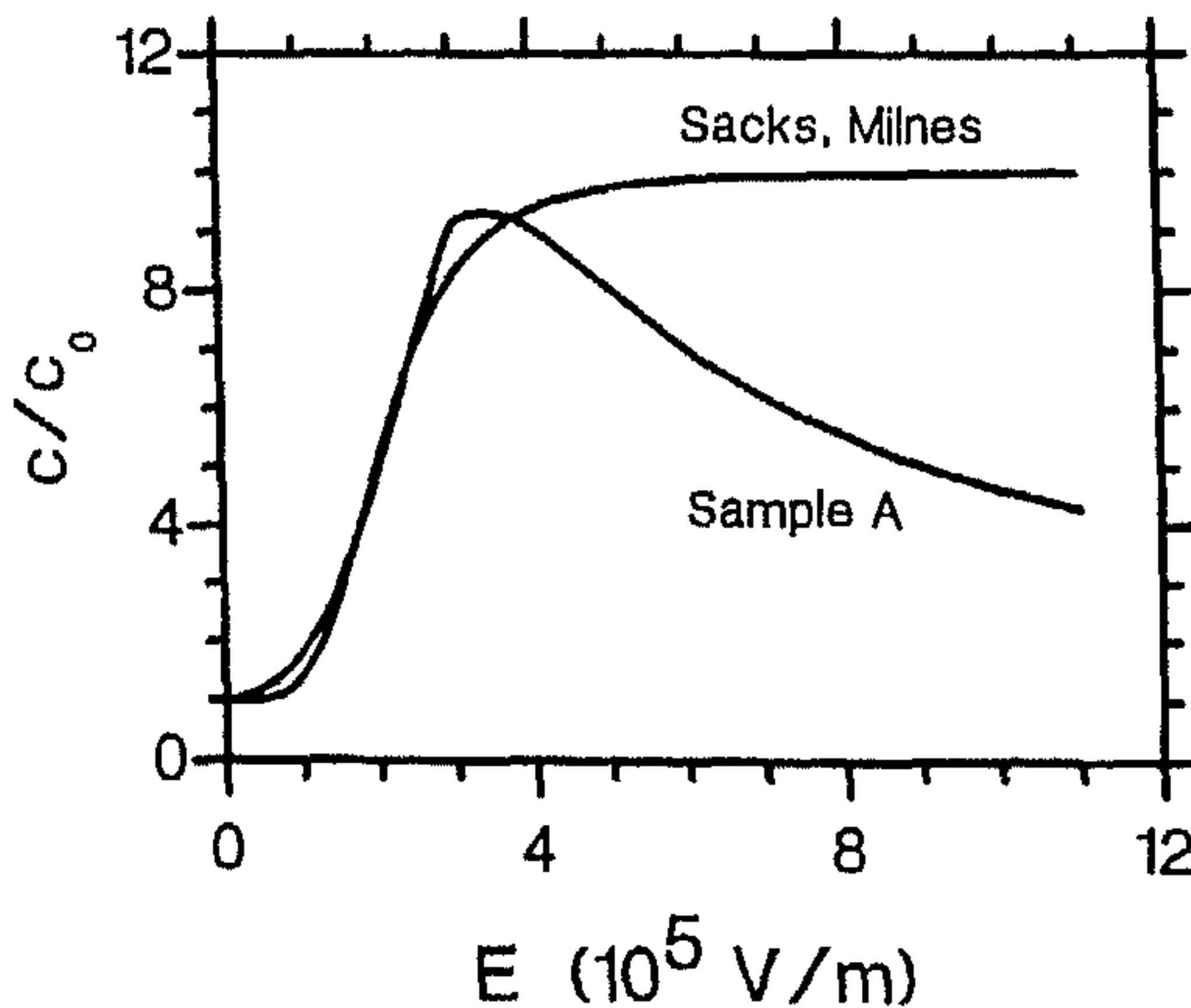
Figure 11. The experimentally determined field dependence of the net capture coefficient c(E) (normalized to c(E = 0) ) of SI-GaAs and the one assumed by Sacks and Milnes [7].
