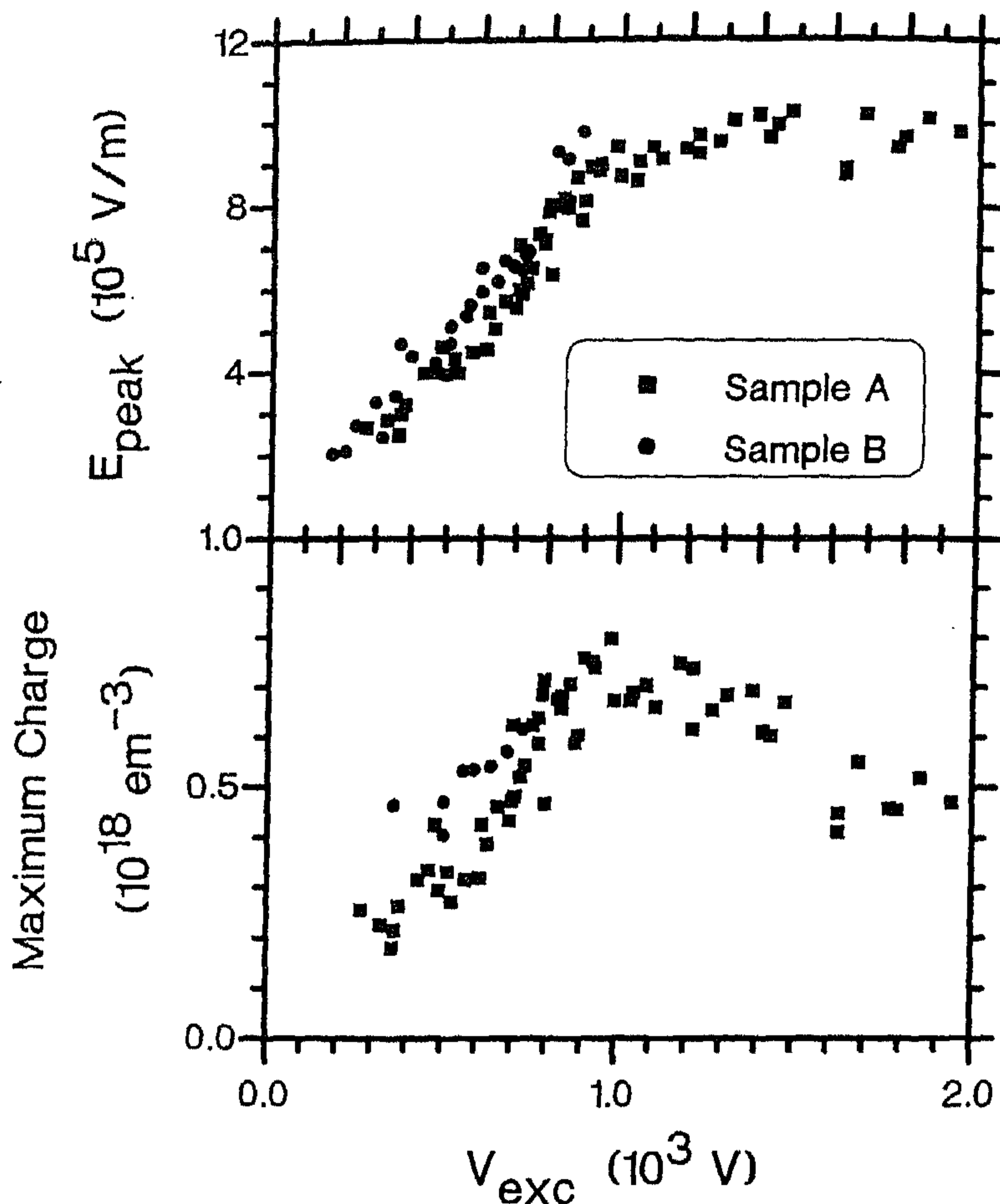
Figure 6. The maximum electric field E_{peak} and maximum space charge of domains as functions of V_{exc} for samples A and B.
