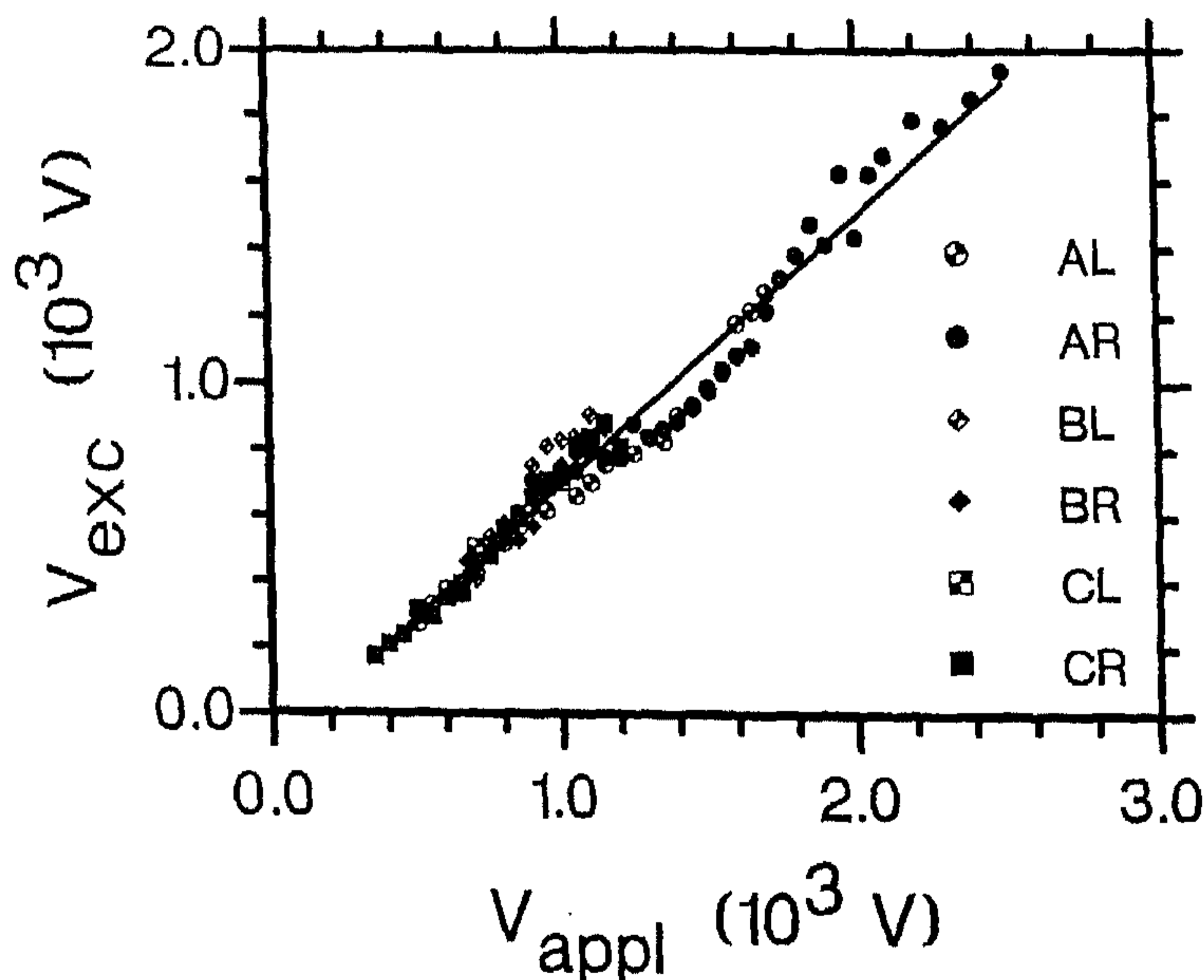
Figure 4. The domain size V_{exc} as a function of the applied voltage V_{appl} for samples A, B and C, with either the left (L) or the right (R) contact as the cathode.
